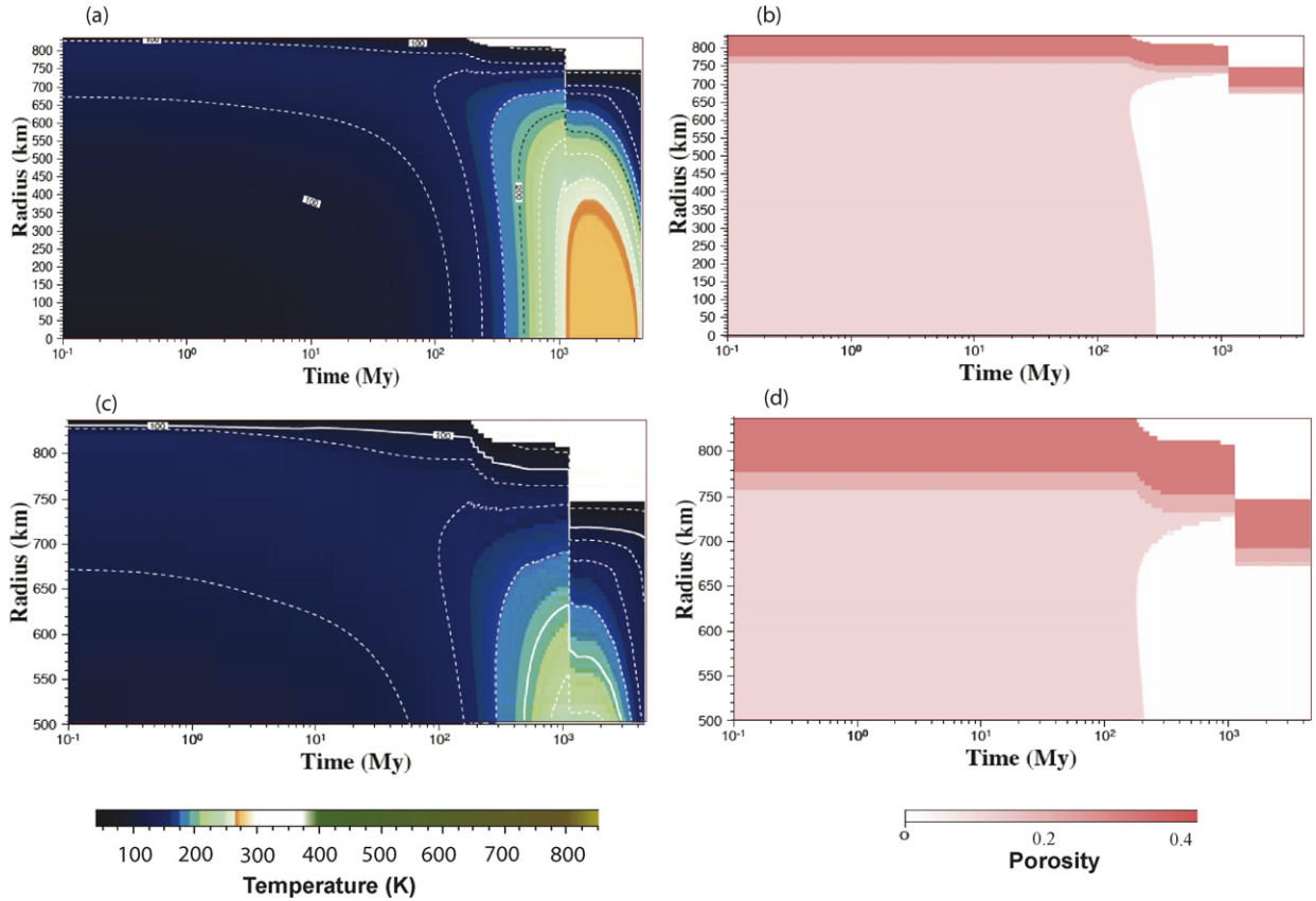
Fig. 6. Same model as in Fig. 5 but with the addition of an initial porosity profile based on Durham et al. (2005) and Kossacki and Leliwa-Kopystynski (1993). (a) Thermal evolution plot (as in Fig. 5); (b) the corresponding porosity evolution; (c) enlargement of the temperature plot for the outer 350 km, and (d) the corresponding enlargement for the porosity evolution. Note the adjustment of radius as the porosity collapses.
